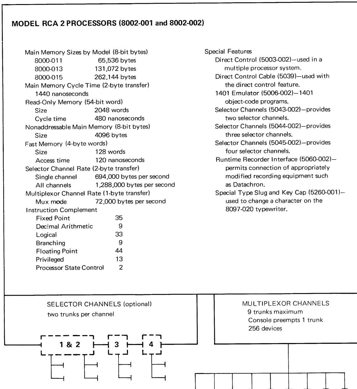
FIGURE 1-6. RCA 2 PROCESSOR DATA
