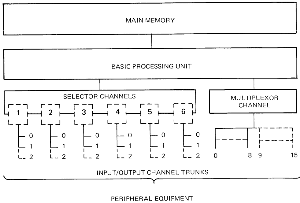
FIGURE 1-1. GENERAL ARRANGEMENT OF RCA SERIES SYSTEM
