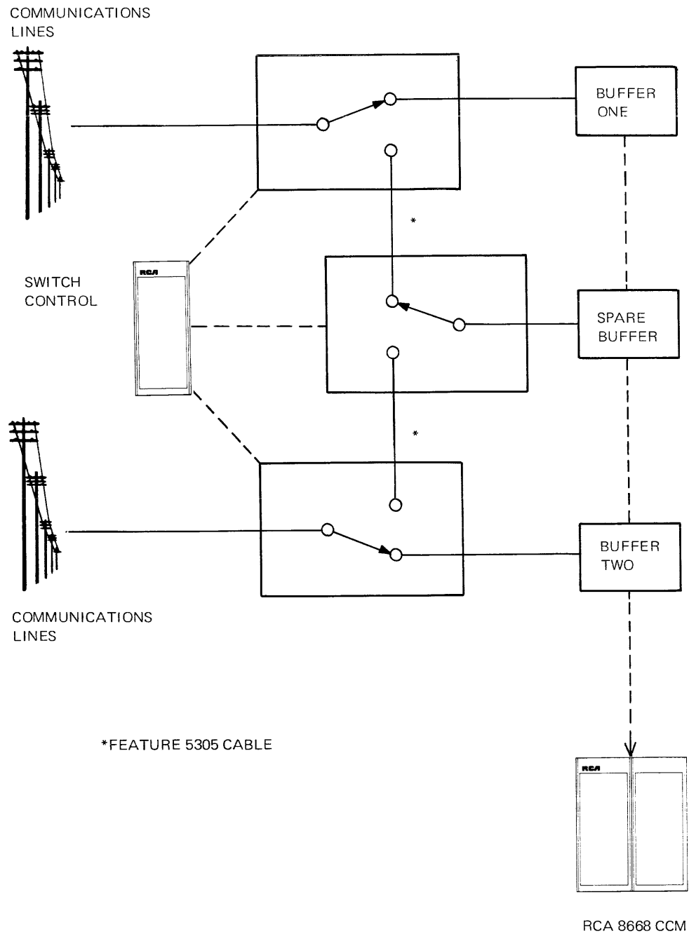
FIGURE 2-6. EXAMPLE OF THREE COMMUNICATIONS SWITCHES CONNECTED CASCADE FOR BACKUP
