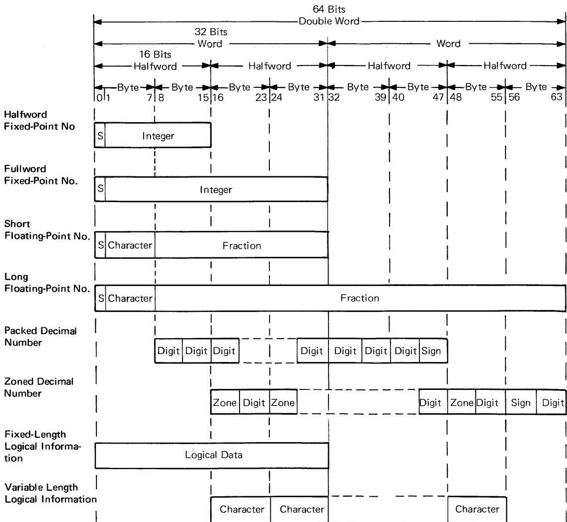
FIGURE 1-3. DATA FORMATS
