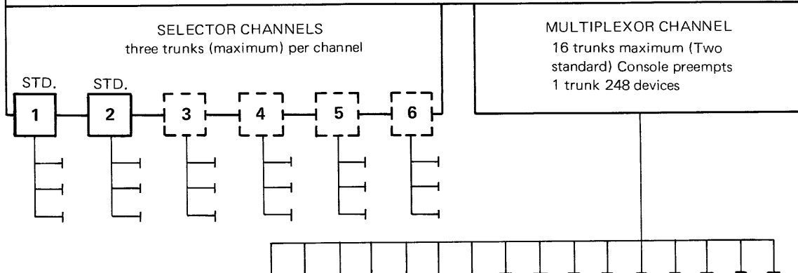
FIGURE 1-10. RCA 6 PROCESSOR DATA
