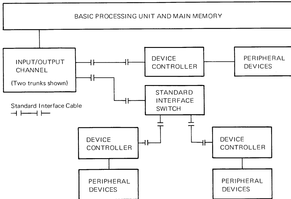
FIGURE 1-2. PERIPHERAL DEVICE TO PROCESSOR ATTACHMENT
