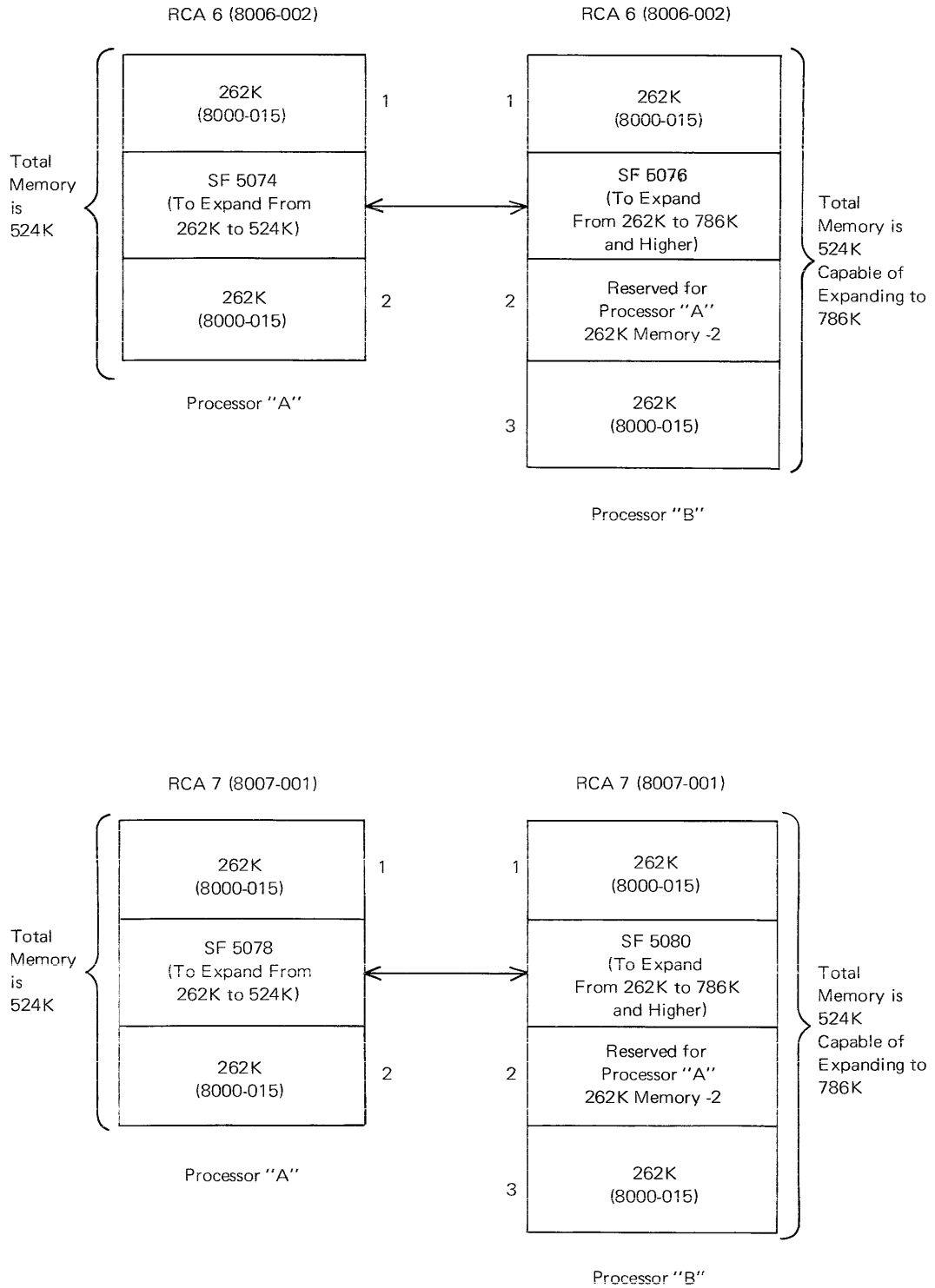
FIGURE 1-4. TYPICAL MEMORY SWITCHING CONFIGURATION FOR THE RCA 6 AND RCA 7.
